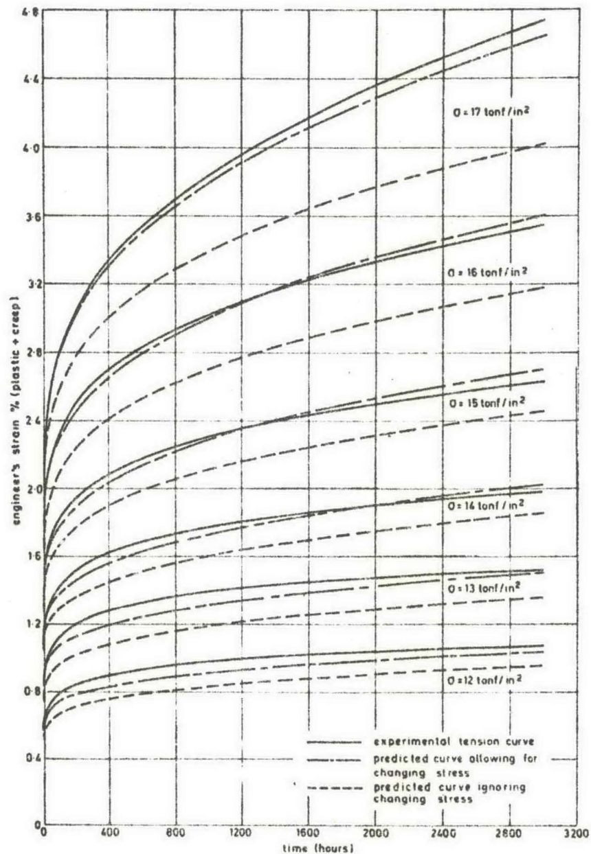
FIG. 13 COMPARISON OF EXPERIMENTAL TENSION CREEP CURVES WITH THOSE PREDICTED FROM TORSION CREEP DATA ON BASIS OF VON MISES FLOW RULE (0.18 PERCENT CARBON STEEL AT 400^{\circ}\text{C} )
